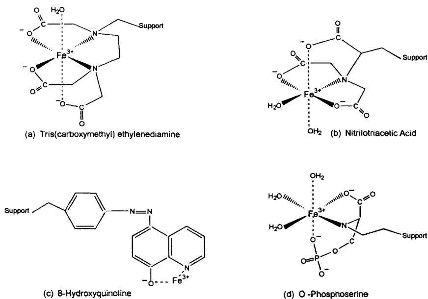
Figure 3. (a) Penta-dentate tris(carboxymethyl)ethylenediamine (TED) complex with Fe(III); (b) Fe(III) complexed to nitilotriacetic acid (NTA) derivatized support; (c) Immobilized 8-hydroxyquinoline complexed with Fe(III); (d) Fe(III) complexed to o-phosphoserine (OPS) derivatized support.
