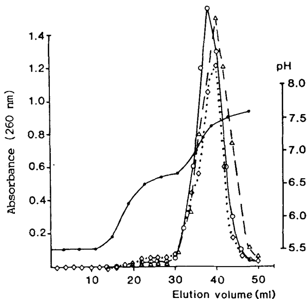
Figure 8. Fe(III)-IMAC elution profiles of adenine nucleotides. AMP (○--○); ADP (△--△); ATP (◇--◇); pH (●--●). (Used with permission from Ref. 16.)
